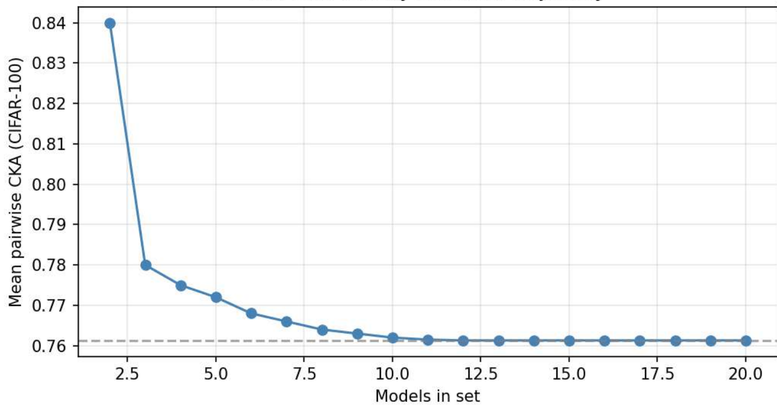
Blur-CNN Greedy Selection Trajectory
