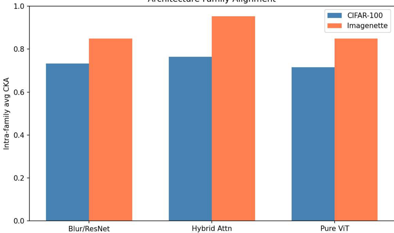
Architecture Family Alignment
