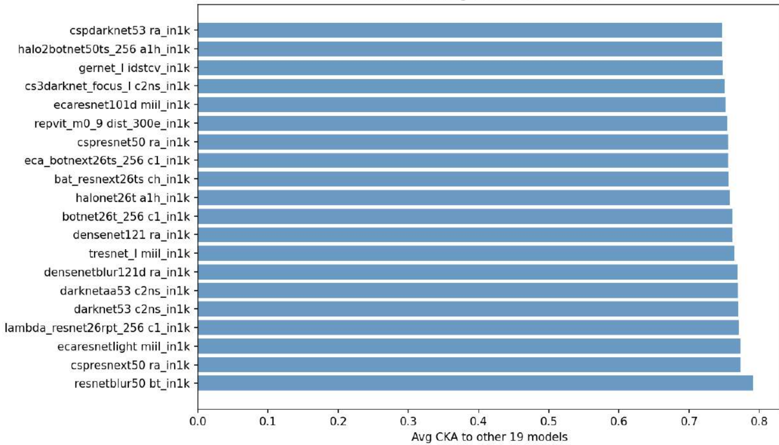
Per-Model Alignment: Blur-CNN Set
