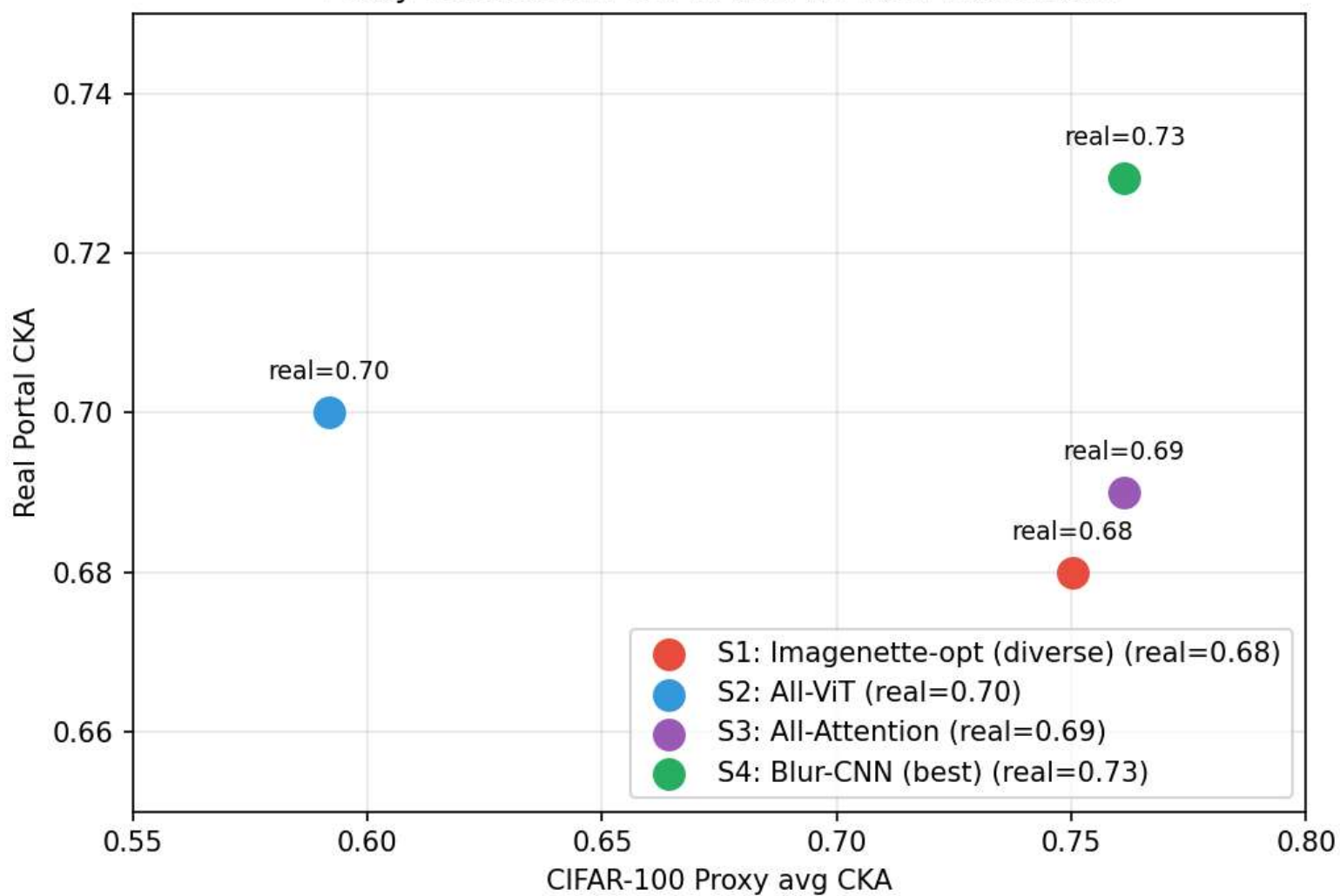
Proxy Calibration: CIFAR-100 vs. Real Evaluation
