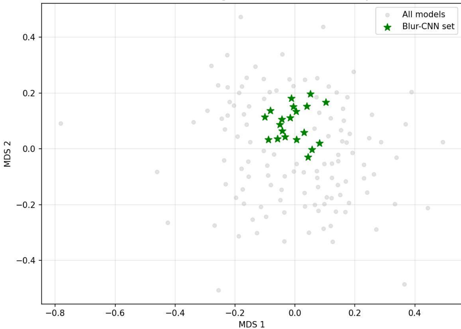
2D MDS Embedding (CIFAR-100 CKA dissimilarity)
